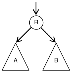
Fig. 4.24. Binary tree
